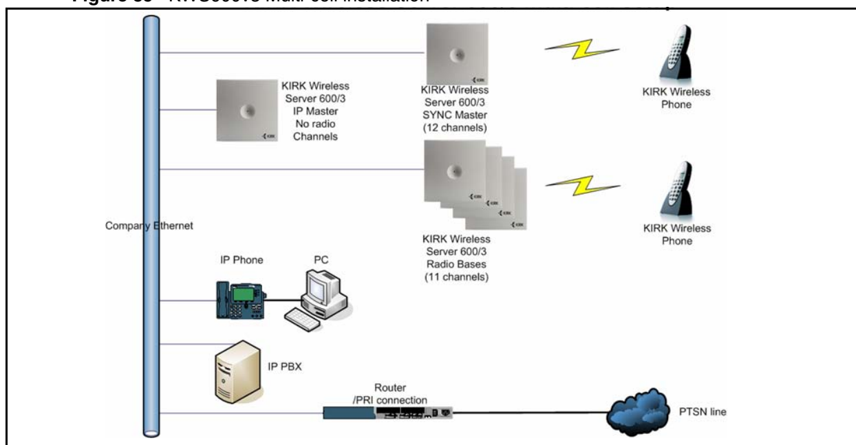
Figure 85 KWS600v3 Multi-cell installation
